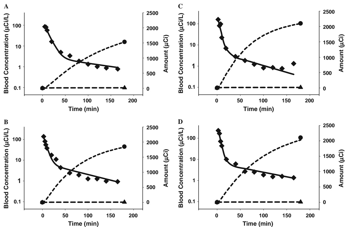
Fig. 5. MEB disposition in Subjects 1 (A), 2 (B), 3 (C) and 4 (D). The curves represent the fit of the pharmacokinetic model based on the scheme depicted in Fig. 2 to the data. The blood concentration-time profiles (diamond) are shown on a log-linear scale (left axes), while bile (filled circle) and urine (triangle) amount vs. time profiles are plotted on a Cartesian scale (right axes). Symbols represent actual data points while lines represent the fit of the model to the data.
