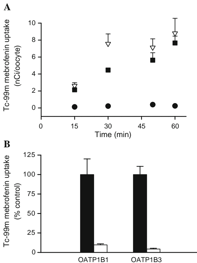
Fig. 3. MEB uptake in Xenopus laevis oocytes expressing human OATP1B1 and OATP1B3. Uptake was measured at room temperature with a MEB concentration of 10 \mu\text{Ci}/\text{ml} (80 pM). Bars and data points represent mean ( \pm SEM) of 5–8 oocytes in a single experiment. Similar results were obtained in an additional independent experiment. A Time course of MEB uptake by uninjected oocytes (control filled circle), OATP1B1- (inverted triangle) and OATP1B3- (filled square) expressing oocytes. B Inhibition of OATP1B1- and OATP1B3-mediated uptake of MEB by rifampicin. Oocytes expressing OATP1B1 and OATP1B3 were incubated for 60 min with MEB (80 pM) in the presence (open bar) and absence (closed bar) of rifampicin (50 \mu\text{M} ). Results are presented as a percentage of untreated oocytes expressing the same protein.
