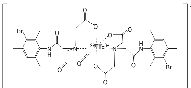
Fig. 1. Structure of MEB. This hepatobiliary imaging agent is an organic anion that consists of two molecules of mebrofenin chelating a central atom of Tc-99m.
