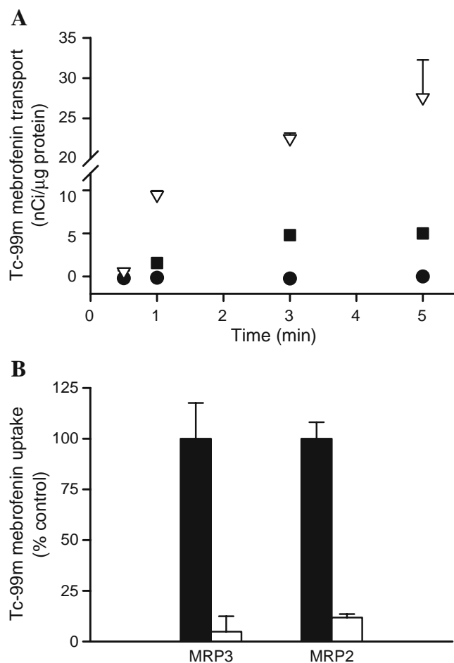
Fig. 4. MEB transport by membrane vesicles prepared from HEK293 cells transiently transfected with MRP2 or MRP3. A A time course of MEB ATP-dependent transport by control (filled circle), MRP2 (inverted triangle) and MRP3 (filled square) membrane vesicles. Transport was measured at 37°C with a MEB concentration of 50 \mu\text{Ci/ml} (0.4 nM). Data points represent mean ( \pm SD) of triplicate determinations in a single experiment. B Inhibition of MRP2- and MRP3-mediated ATP-dependent transport of MEB. Membrane vesicles were incubated for 3 min with MEB (0.4 nM) in the presence (open bar) and absence (closed bar) of E 2 17 \beta G (100 \mu\text{M} ) for MRP3 inhibition, and MK571 (50 \mu\text{M} ) for MRP2 inhibition. Results are expressed as a percentage of untreated membranes. Bars represent mean ( \pm SD) of triplicate determinations in a single experiment.
