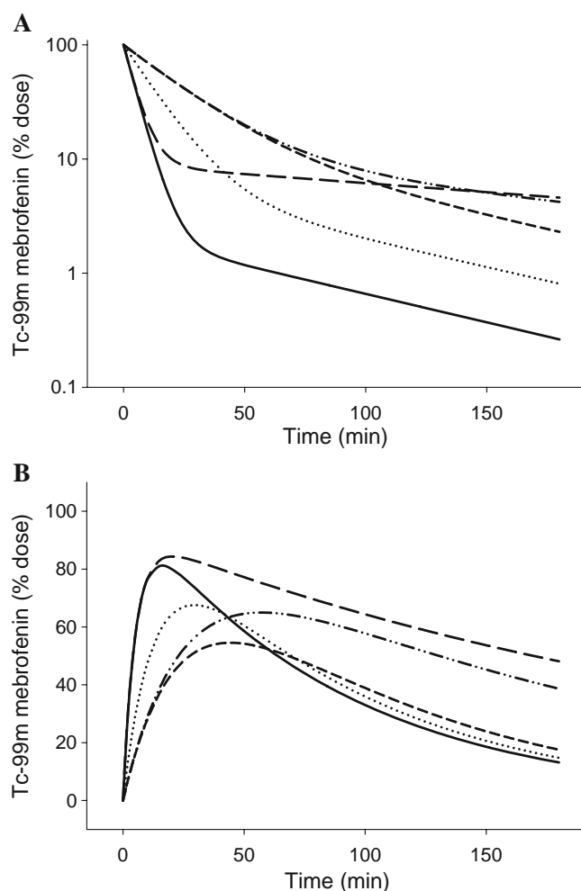
Fig. 6. Simulations of MEB disposition in blood and liver of patients with altered hepatic uptake and/or excretion consistent with hyperbilirubinemia, inflammation-induced cholestasis and obstructive cholestasis. Predicted modifications in the blood concentration-time profiles ( A ) and in the hepatic exposure over time ( B ) due to various liver pathologies. The solid line represents the simulated profile in healthy volunteers. Simulations were designed to reflect changes due to mild hyperbilirubinemia [ dotted line ; 2.5-fold impaired hepatic uptake ( k_{12} ) of MEB], intermediate hyperbilirubinemia [ dashed line ; 5-fold impaired hepatic uptake ( k_{12} ) of MEB], inflammation-induced cholestasis [ dash-dotted line ; 5-fold impaired hepatic uptake ( k_{12} ) of MEB with 2-fold impaired biliary excretion ( k_{20} )], and obstructive cholestasis [ long dashed line ; 3-fold impaired biliary excretion ( k_{20} ) with induction of hepatic basolateral excretion (5-fold increase in k_{21} )].
