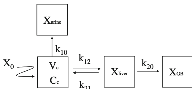
Fig. 2. Scheme of the pharmacokinetic model describing the disposition and elimination of MEB in humans. X_0 represents the IV bolus dose. C_c is the concentration of MEB in the central compartment (blood) and V_c is the central compartment volume. All other compartments were modeled as amounts [in urine ( X_{urine} ), in the hepatocytes ( X_{liver} ) and in the gallbladder (GB) estimated as duodenal bile corrected for EF ( X_{GB} )]. All rate constants were assumed to be first-order: k_{12} represents hepatic basolateral uptake, k_{21} represents hepatic basolateral excretion, k_{20} represents hepatic canalicular excretion, and k_{10} represents the rate constant for renal elimination.
